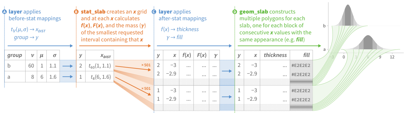
Fig. 2: Flow of data through the visualization construction pipeline for a Helske [18]-style interval+density plot using ggdist::stat_slab . The layer , part of ggplot2 , applies initial aesthetic mappings, translating input data into columns understood by stat_slab , which then constructs a larger data frame containing evaluations of distribution functions over an x grid for each distribution (the user can specify the grid size if needed; the default size is 501). Then, layer applies a second set of aesthetic mappings, and geom_slab uses the final data frame to construct the plot.
