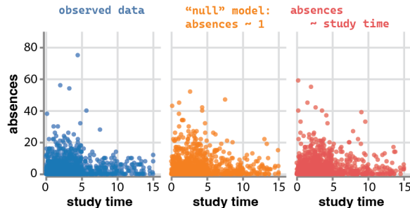
Fig. 2: Model check showing what the data would look like if absences was not associated with study_time (orange) vs if it was (red). Predictions from the two models look very similar.
